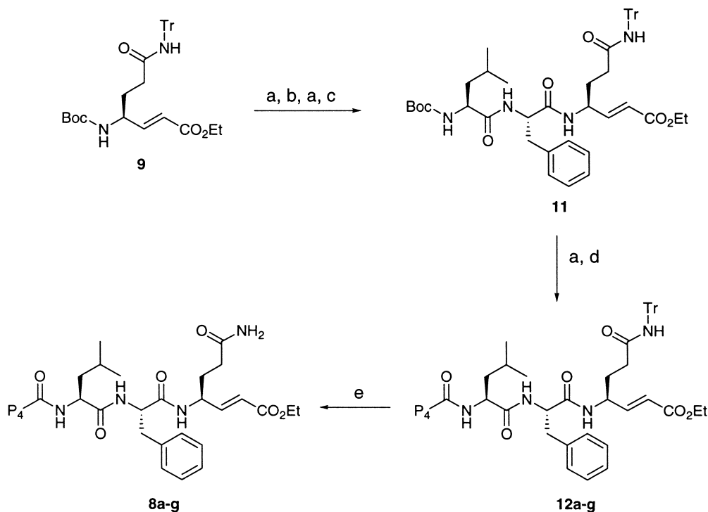
Scheme 2. Reagents and conditions (Tr = CPh 3 ): (a) HCl in 1,4-dioxane, 23 °C, 2 h; (b) 1.0 equiv Boc-L-Phe-OH, 1.5 equiv HOBt, 3.0 equiv NMM, 1.5 equiv EDC, CH 2 Cl 2 , 23 °C, overnight, 85%; (c) 1.2 equiv Boc-L-Leu-OH, 1.5 equiv HOBt, 3.0 equiv NMM, 1.5 equiv EDC, CH 2 Cl 2 , 23 °C, overnight, 87%; (d) excess RCO 2 H and Et 3 N, CH 2 Cl 2 , 0 °C, 30 min or excess RCO 2 H, HOBt, NMM and EDC, CH 2 Cl 2 , 23 °C, overnight; (e) excess ( i -Pr) 3 SiH, 1:1 TFA:CH 2 Cl 2 , 23 °C, 30 min.
