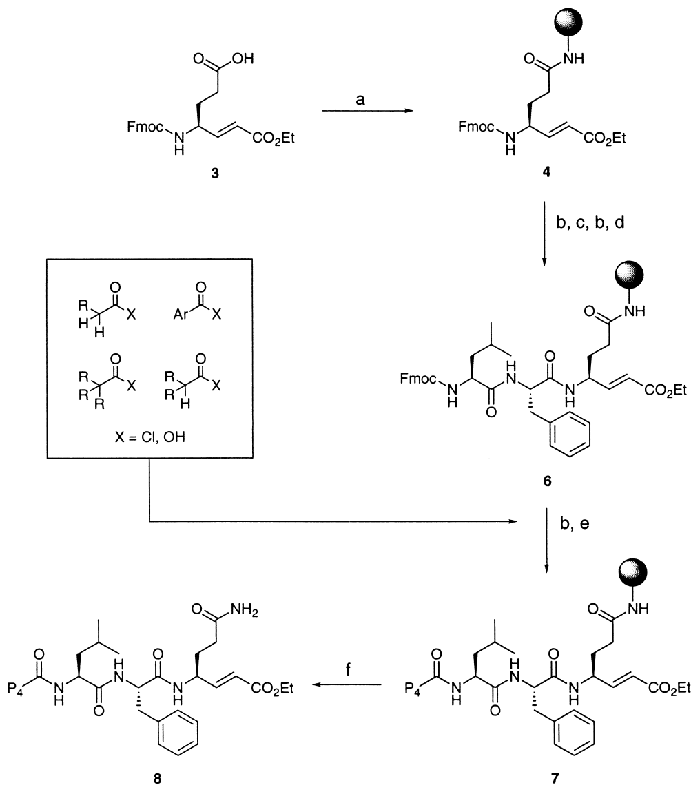
Scheme 1. Reagents and conditions: (a) 0.2 equiv solid-supported Rink-Amide linker, 2.0 equiv DIEA, 0.10 equiv HOBt, 1.0 equiv PyBOP, DMF, 23 °C, 1 h; (b) 2% DBU in CH 2 Cl 2 , 23 °C, 30 min; (c) 5.0 equiv Fmoc-L-Phe-OH, 10.0 equiv collidine, 5.0 equiv HATU, DMF, 23 °C, 1 h; (d) 5.0 equiv Fmoc-L-Leu-OH, 10.0 equiv collidine, 5.0 equiv HATU, DMF, 23 °C, 1 h, 2 times; (e) excess RCO(O)Cl and collidine, CHCl 3 , 23 °C, 1 h or excess RCO 2 H, DIEA, HATU, DMF, 23 °C, 1 h, 2 times; (f) 95:5 TFA:H 2 O, 23 °C, 1 h.
